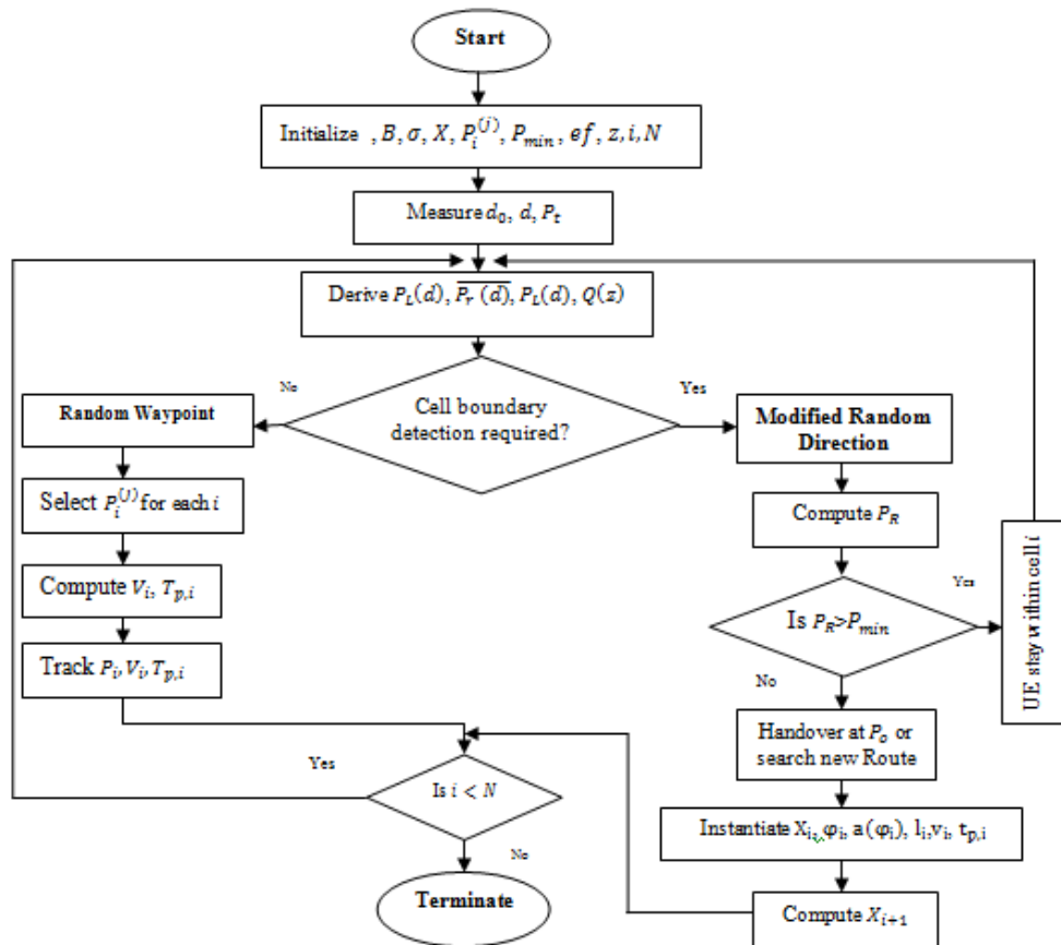
Fig.3. Modeling Pseudo-Stochastic Mobility Tracking Protocol
