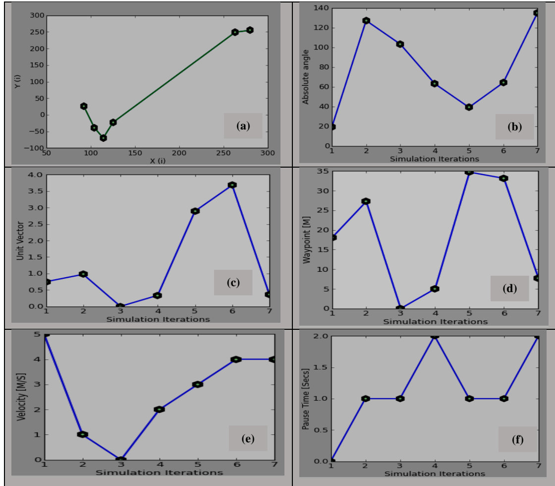
Fig.9. Variations of Mobility Vectors
