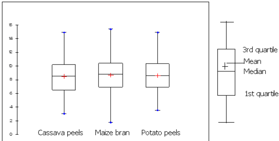
Fig.1. Box plots comparing growth performance (SL) performance of different test diets.
