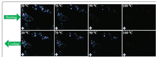
Figure 2: Micrographs showing effect of temperatures on molecular ordering of rGO crystallites. (Image size 68x52 μm)
