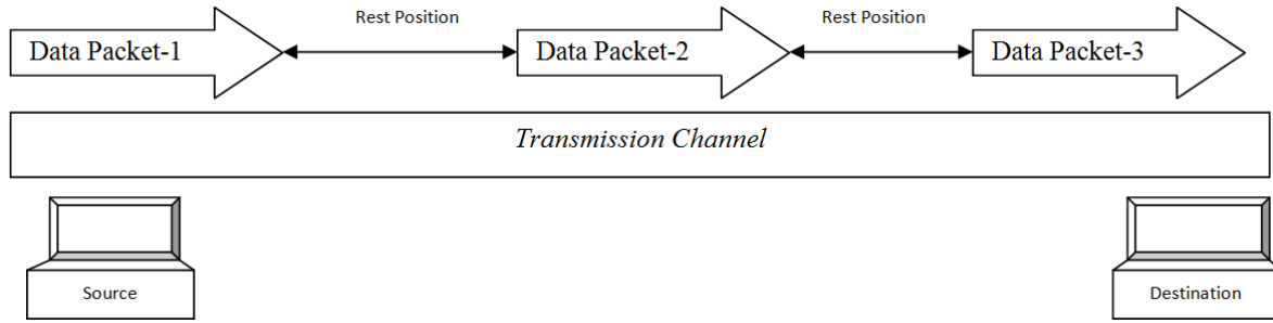
Figure 14. TCP Pacing.
